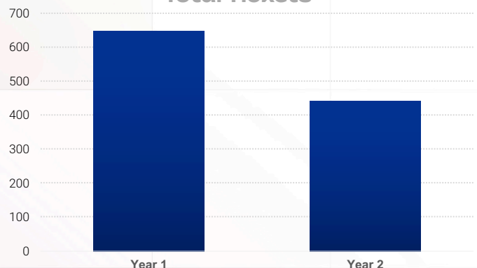
Total Tickets
