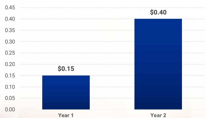
Token Price
