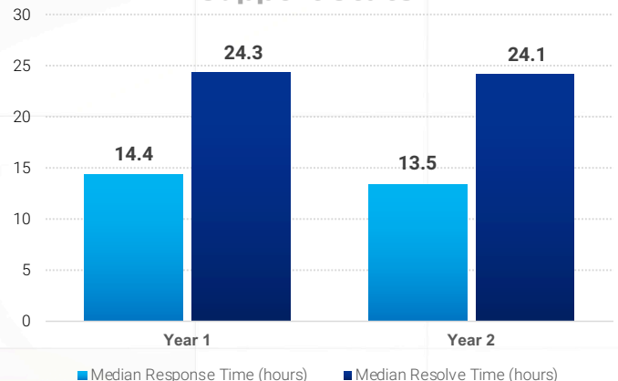
Support Stats
